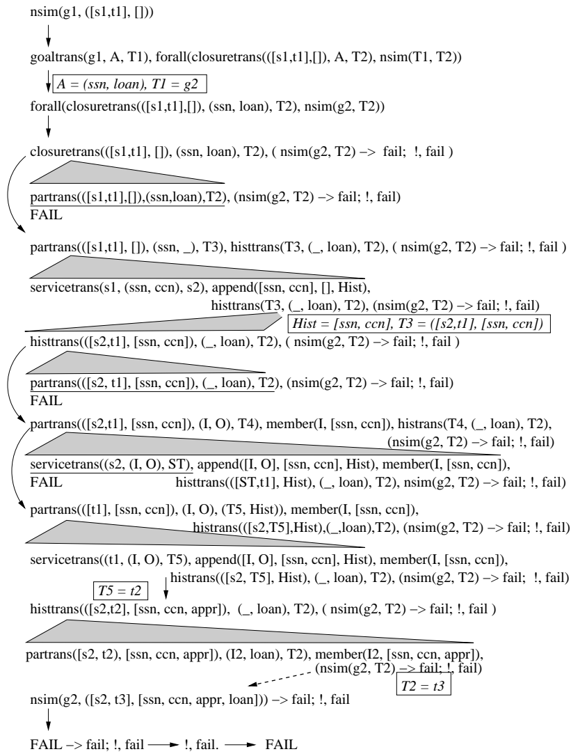
Figure 4.2: Execution tree.
